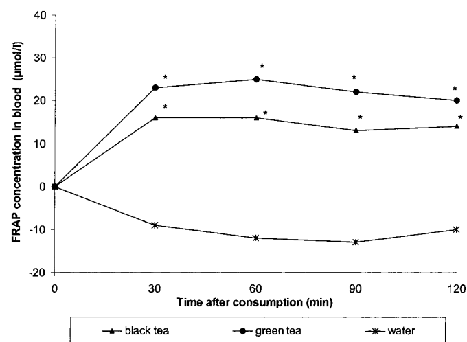
FIGURE 2 Changes in plasma FRAP activity ( \mu mol/L) over 120 min after a single dose of black tea, green tea and water. * P < 0.001 , tea versus water
